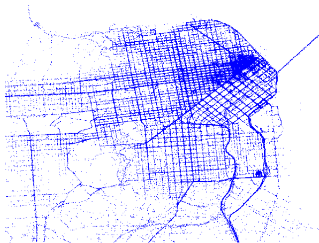
Figure 1. San Francisco taxi measurement locations for a single day, observed at a rate of once per minute.
